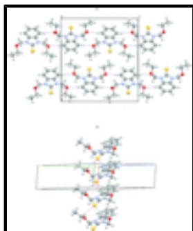
Fig. 2. Packing diagram with two different views; hydrogen bonds drawn as dashed lines.
